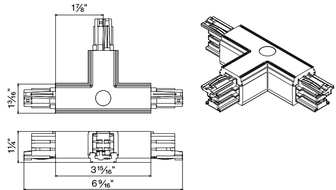
T-FEED
