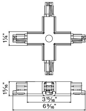
X-FEED
