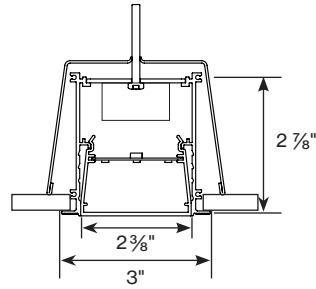
RECESSED trimless
