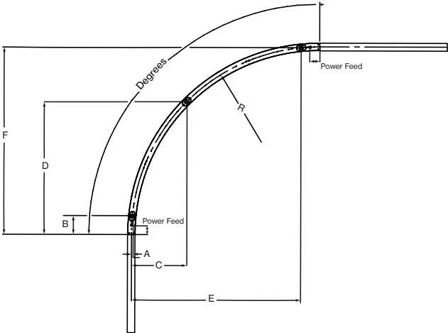
CURVE MOUNTING POINT DIMENSIONS
